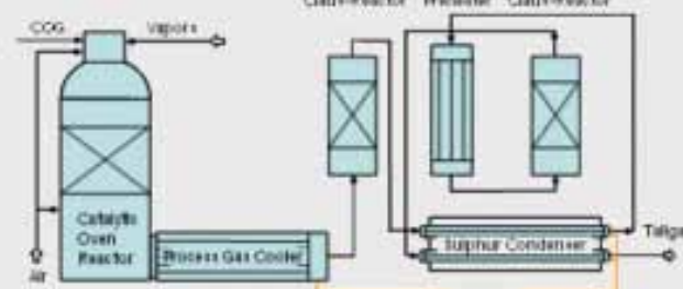
Claus plant with ammonia cracking
